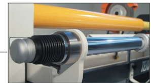
Front unwinding shaft with brake to rewinding log rolls
